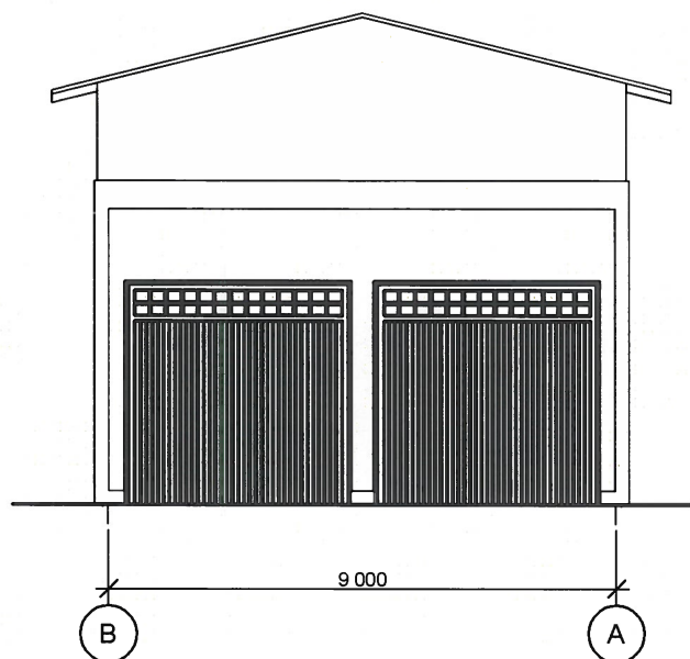
Fatada in axele B-A
