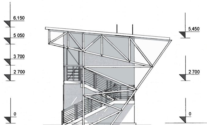
Fatada laterala
