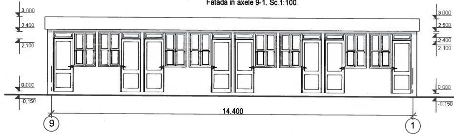
Fatada in axele 9-1, Sc.1:100.
