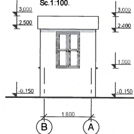
Fatada in axele B-A, Sc.1:100.
