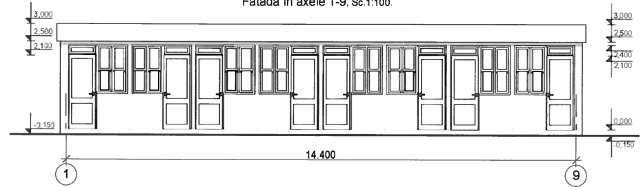
Fatada in axele 1-9, Sc.1:100.
