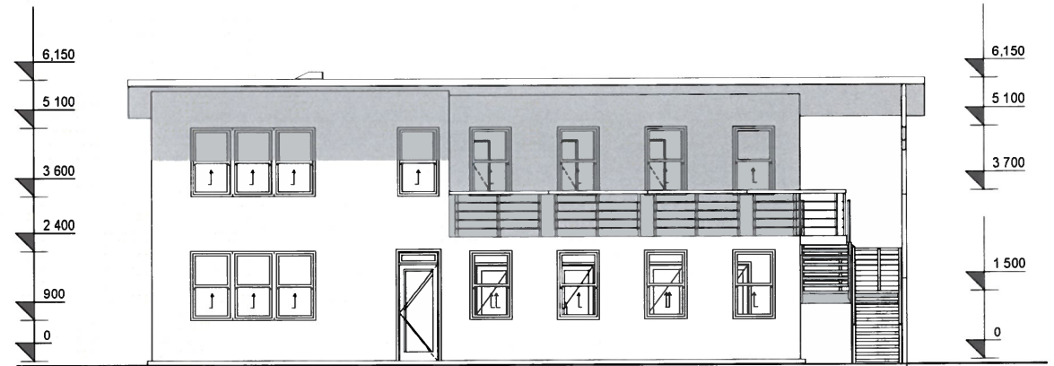
Fatada principala
