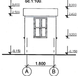
Fatada in axele A-B, Sc.1:100.
